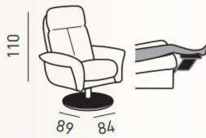
Armchair Relax Swivel with one aluminium central axle (incorated footrest)
